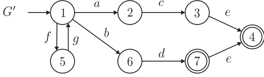
Fig. 3. Example generator G' that violates observation consistency .
