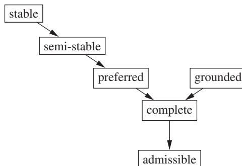
Figure 1. Overview of argumentation semantics and their relations.
