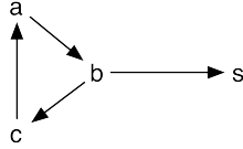
Figure 2.9: Framework F .
