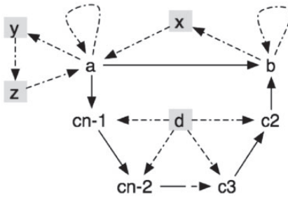
FIGURE 11. F\cup H .
