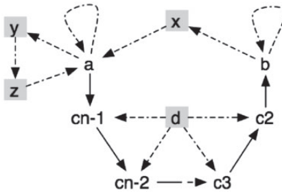
FIGURE 12. G\cup H .
