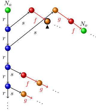
Figure 6: A collapsing obtained from the one depicted in Figure 5.
