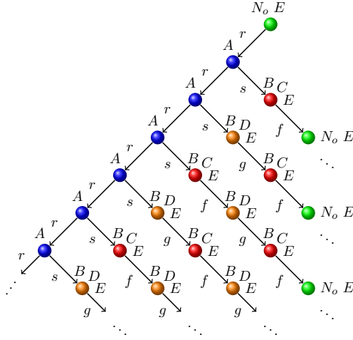
Figure 3: Unraveling of the model displayed in Figure 2.
