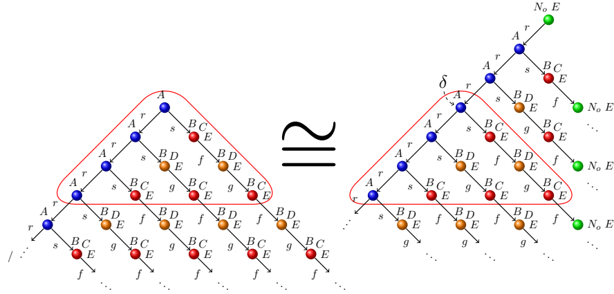
Figure 11: Forest quasi-model (right) and according 3-secure replacement for \delta (left).
