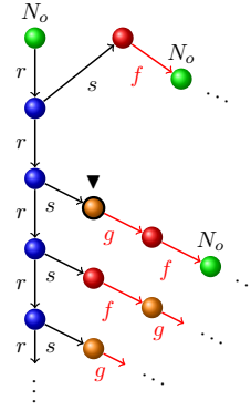
Figure 5: In the first collapsing step we just rename elements to promote the focus from Figure 4 to a root.
