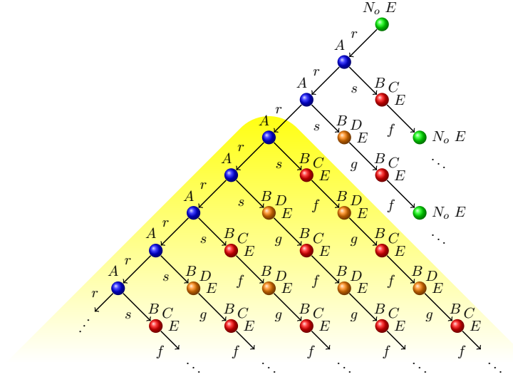
Figure 12: Result of replacing the element \delta by the 3-secure replacement depicted in Figure 11. The inserted component is highlighted.
