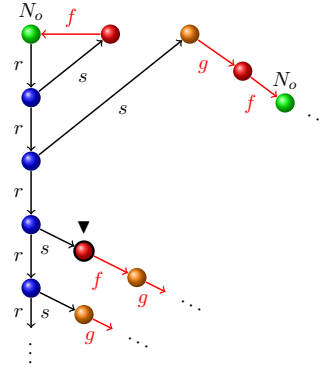
Figure 7: A collapsing obtained by using the second case of Definition 17 on the collapsing from Figure 6.
