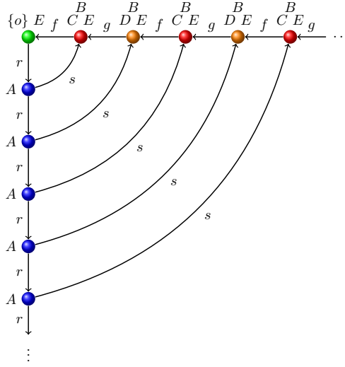
Figure 8: Result of collapsing the unraveling from Fig. 3. The infinitely many new root elements are displayed in the top line.
