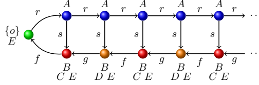
Figure 2: Knowledge base for our running example and a representation of a model for the knowledge base.
