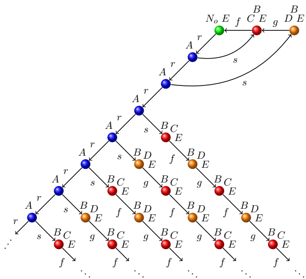
Figure 13: Result of collapsing the forest quasi-model displayed in Figure 12.
