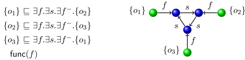
Figure 1: Example knowledge base \mathcal{K} and a representation for a model, where the three elements in the s -cycle are so-called new nominals .
