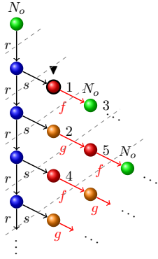
Figure 4: An initial collapsing for the unraveling depicted in Figure 3.
