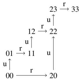
Figure 1: Visualization of the instance from Exercise 3.3
