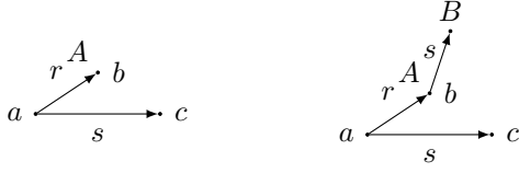
Figure 3: Canonical Models with \mathcal{A} = \{r(a, b), A(b), s(a, c)\} and \mathcal{T} = \{A \subseteq \exists s.B\}
