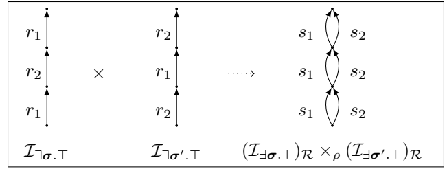
Figure 4: Product of (\mathcal{I}_{\exists\sigma.\top})_{\mathcal{R}} \times_{\rho} (\mathcal{I}_{\exists\sigma'.\top})_{\mathcal{R}} with \sigma = r_1 r_2 r_1 , \sigma' = r_2 r_1 r_2 and \mathcal{R} = \{r_1 \sqsubseteq s_1, r_1 \sqsubseteq s_2, r_2 \sqsubseteq s_1, r_2 \sqsubseteq s_2\} .
