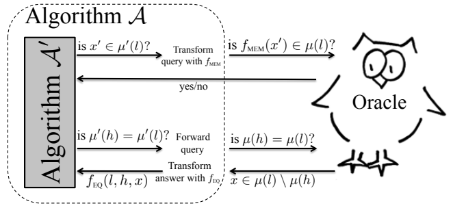
Figure 6: Learning by reduction algorithm
