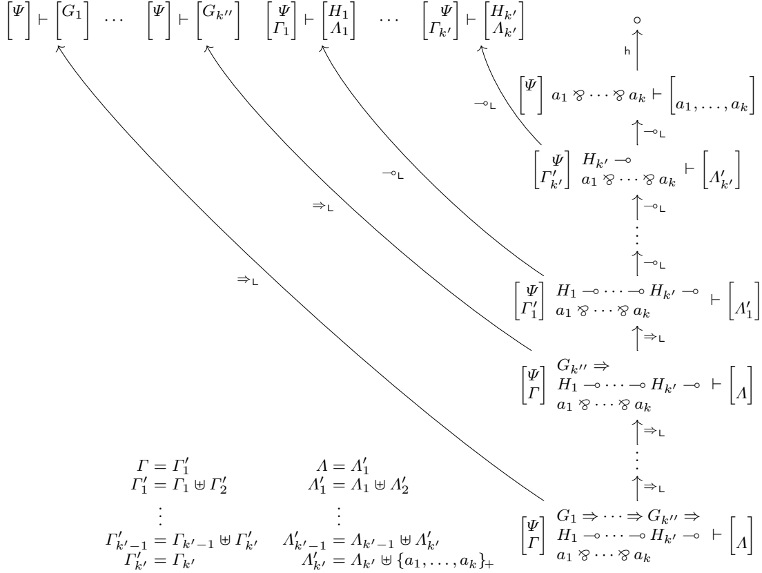
Fig. 6 Clause reduction left inference rule \delta_{\perp}
