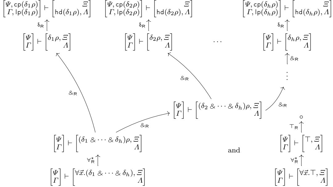
Fig. 4 Goal reduction right inference rule G_R when h > 0 and h = 0
